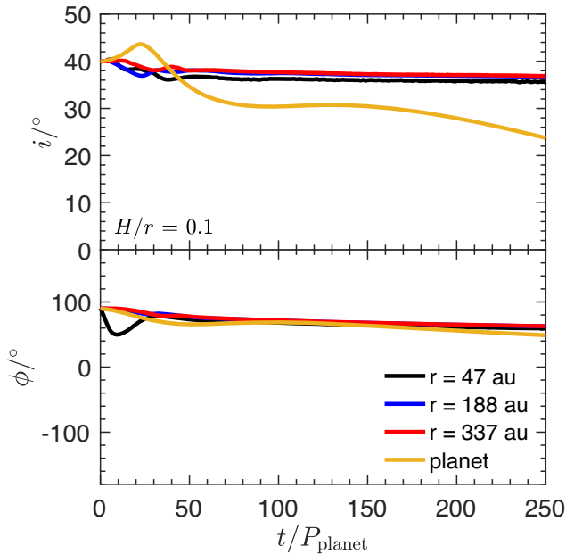
Figure 8. Evolution of the inclination, i , and longitude of the ascending node, \phi , both as a function of time for two different disc aspect ratios. Left-hand panel: H/r = 0.1 (run5 from Table 3). Right-hand panel: H/r = 0.05 (run4). The disc is evaluated at three radii, 47 au (black), 188 au (blue), and 337 au (red). The planet is given by the yellow lines.
